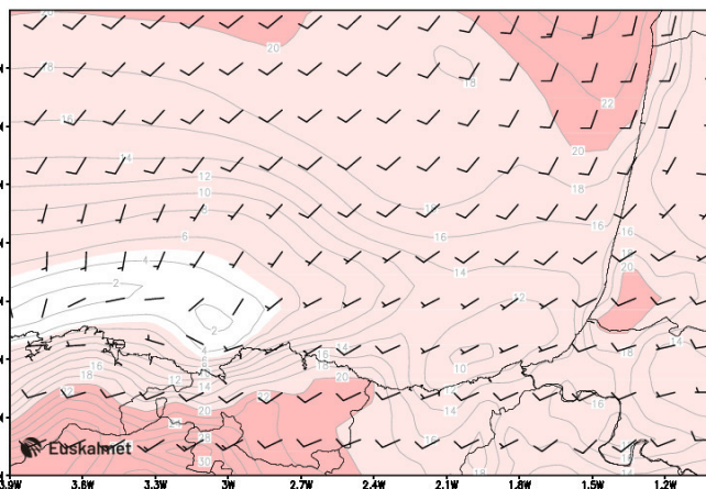
Haizea azalean (km/h) 2024/02/13 12:00 Viento superficial (km/h)
