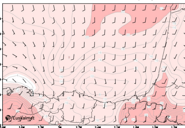
Haizea azalean (km/h) 2024/02/14 12:00 Viento superficial (km/h)
