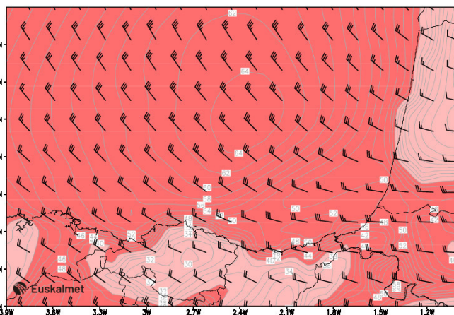
Haizea azalean (km/h) 2024/02/12 12:00 Viento superficial (km/h)
