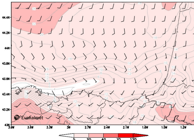
Haizea azalean (km/h) 2024/02/10 12:00 Viento superficial (km/h)
