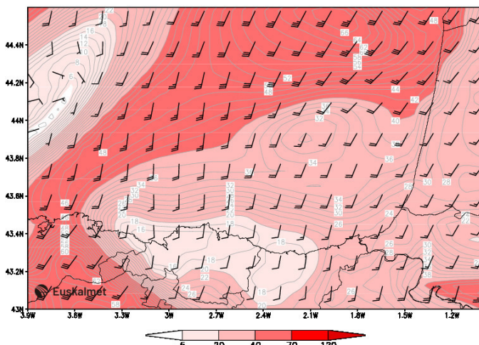
Haizea azalean (km/h) 2024/02/09 12:00 Viento superficial (km/h)
